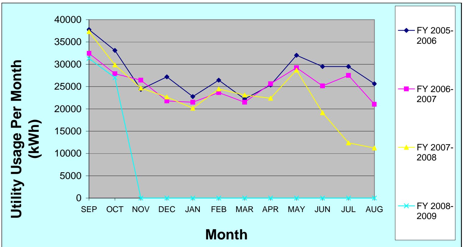
Usage Trend Graph- Anthony Elementary School Cafeteria 4 Year Trend- Electricity Usage
