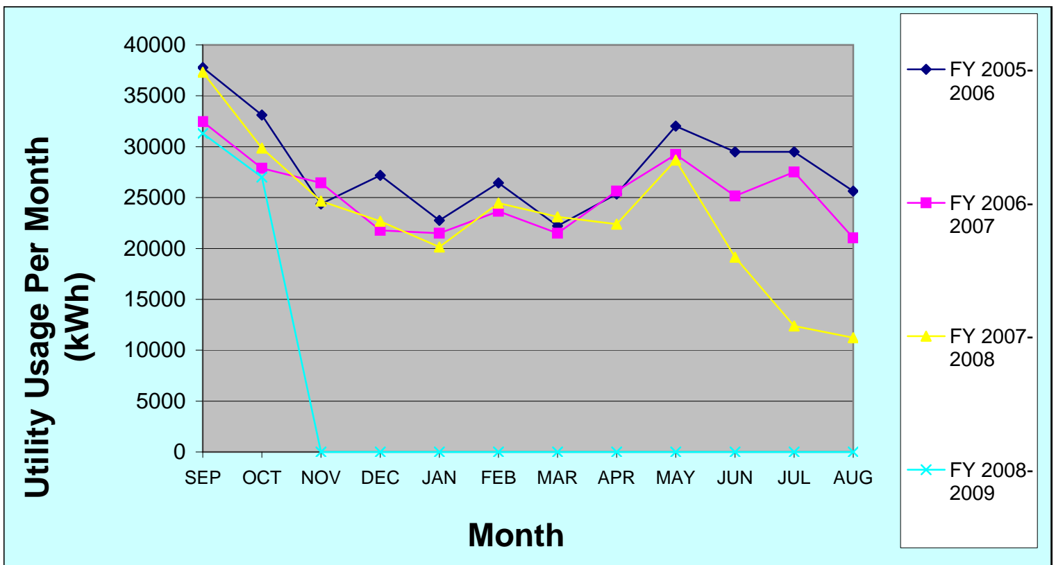
Usage Trend Graph- Anthony Elementary School 4 Year Trend- Electricity Usage
