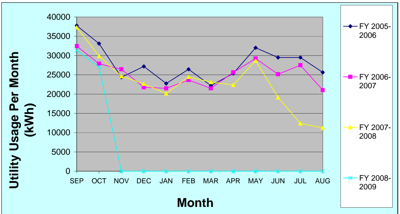
Usage Trend Graph- Anthony Middle/High School Cafeteria 4 Year Trend- Electricity Usage
