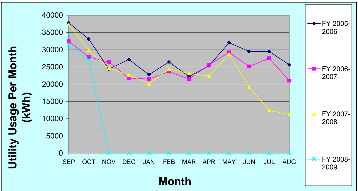
Usage Trend Graph- Anthony High School 4 Year Trend- Electricity Usage
